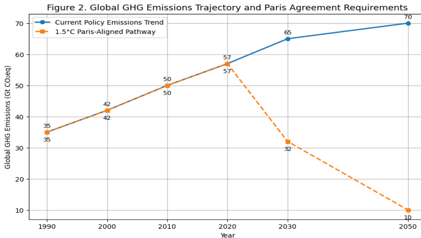
Figure 2: Global GHG emissions trajectory and Paris agreement requirements (1990-2050)
